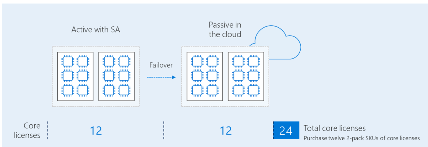
This figure shows an example of licensing an active primary SQL Server 2017 database with Software Assurance and a passive secondary database hosted in the cloud.
